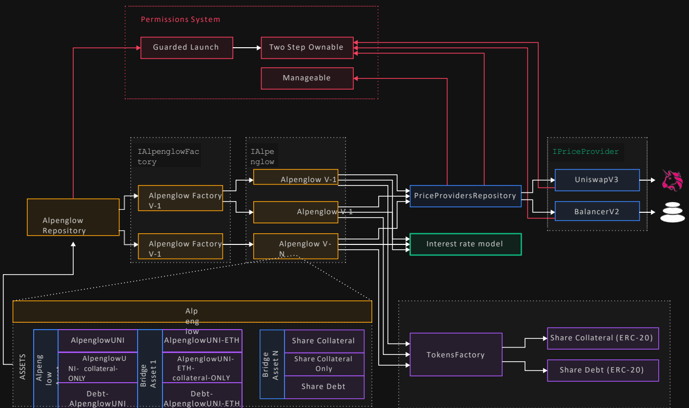
Fig. 1Alpenglow protocol architecture
